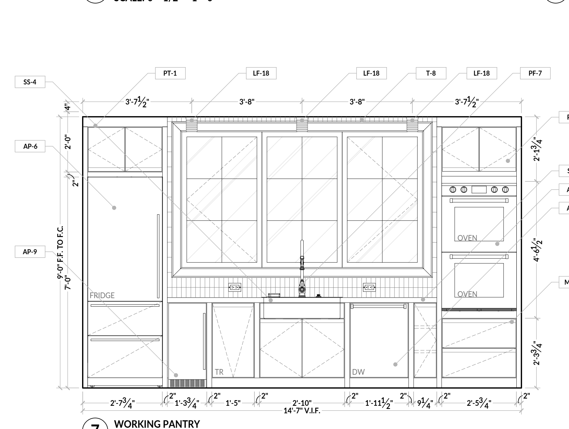
7 WORKING PANTRY SCALE: 0' - 1/2" = 1' - 0"
