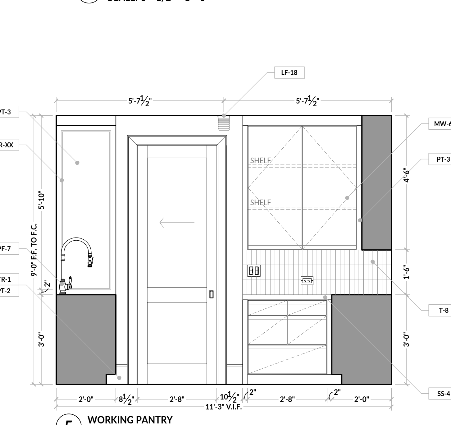
5 WORKING PANTRY SCALE: 0' - 1/2" = 1' - 0"
