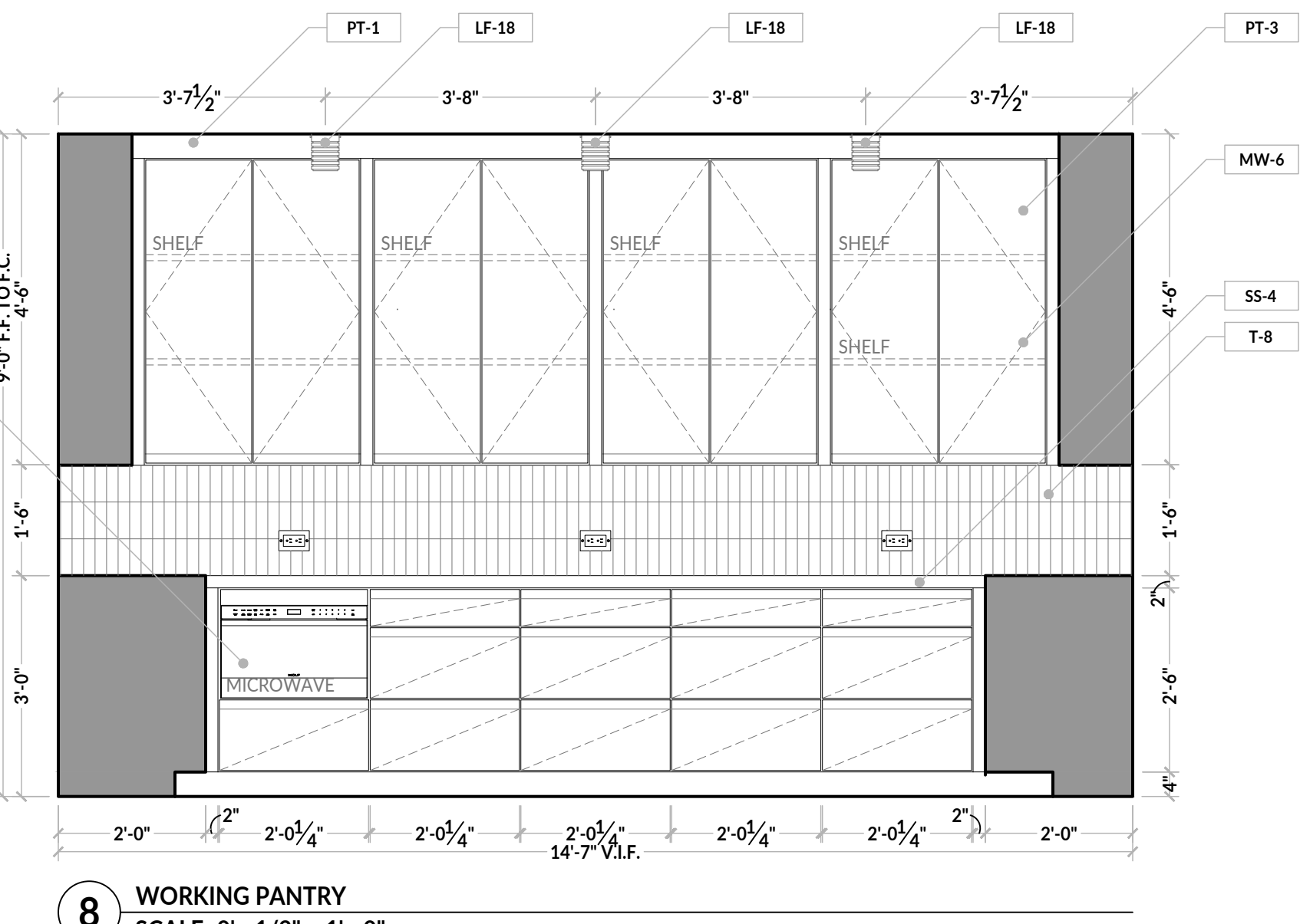
8 WORKING PANTRY SCALE: 0' - 1/2" = 1' - 0"
