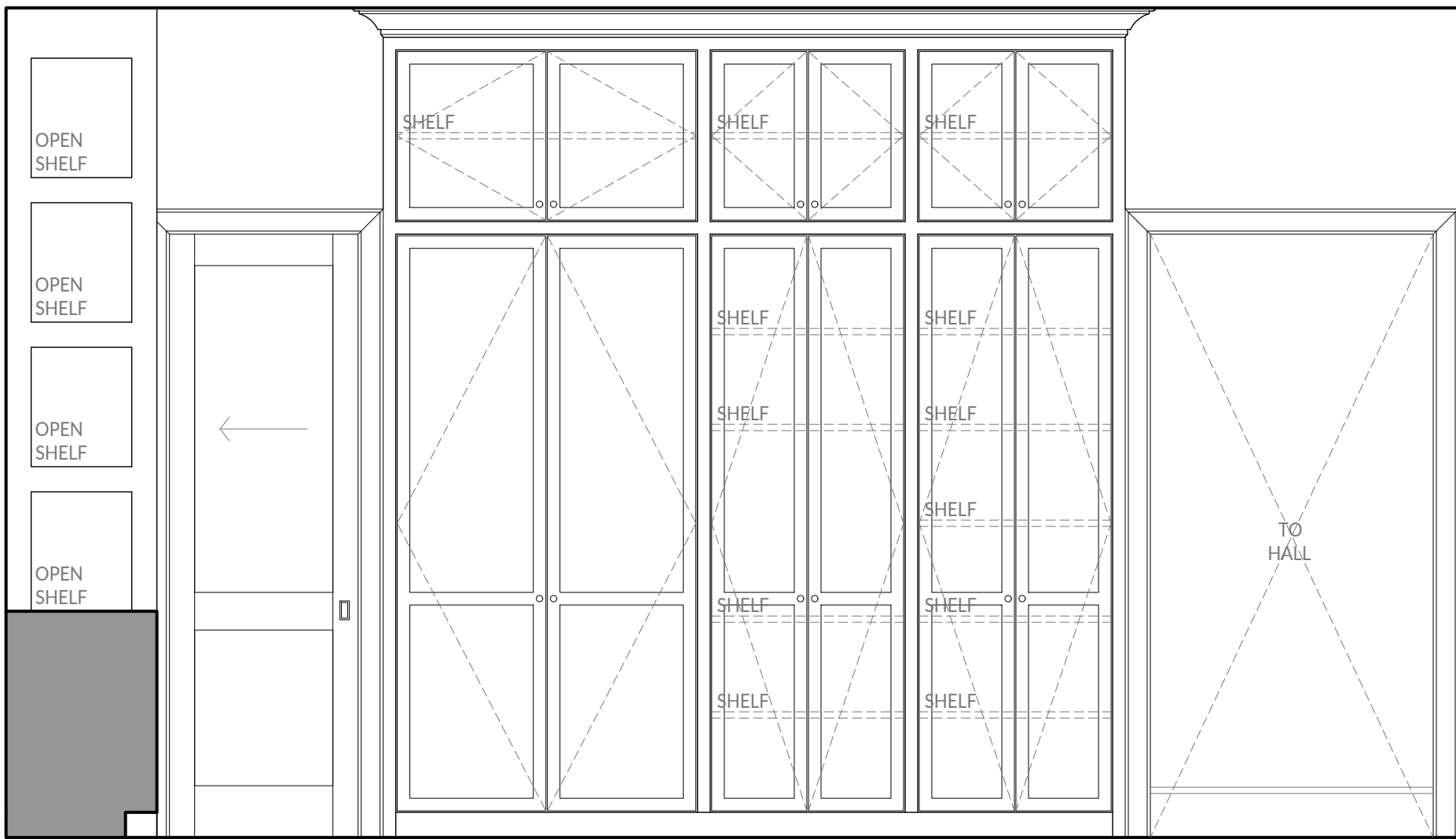
1 KITCHEN SCALE: 0' - 1/2" = 1' - 0"
