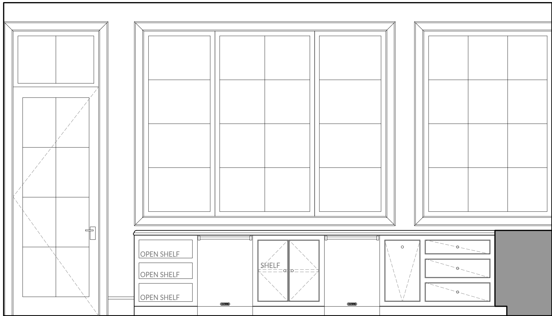
8 KITCHEN SCALE: 0' - 1/2" = 1' - 0"
