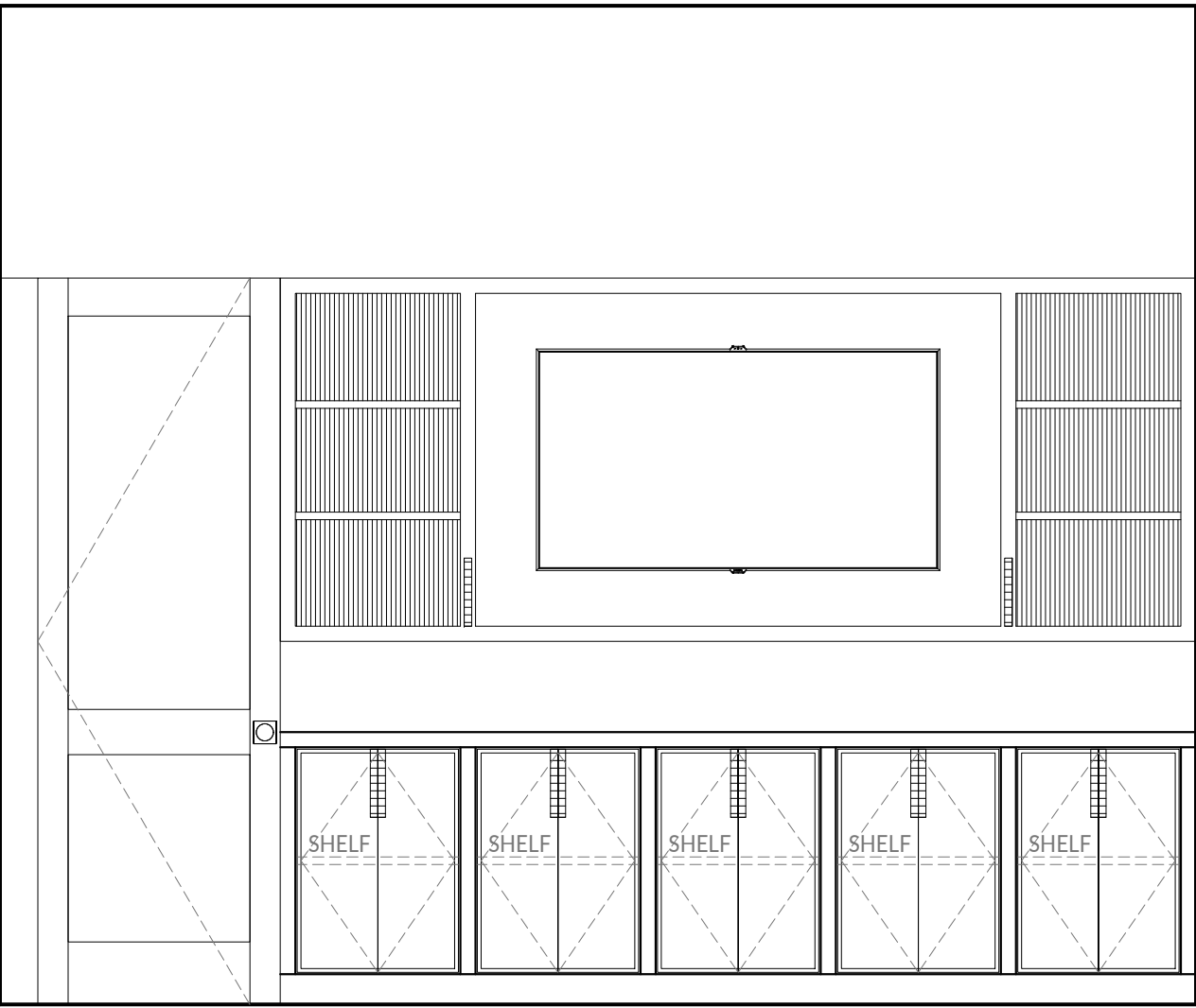
5 GAME ROOM SCALE: 0' - 1/2" = 1' - 0"
