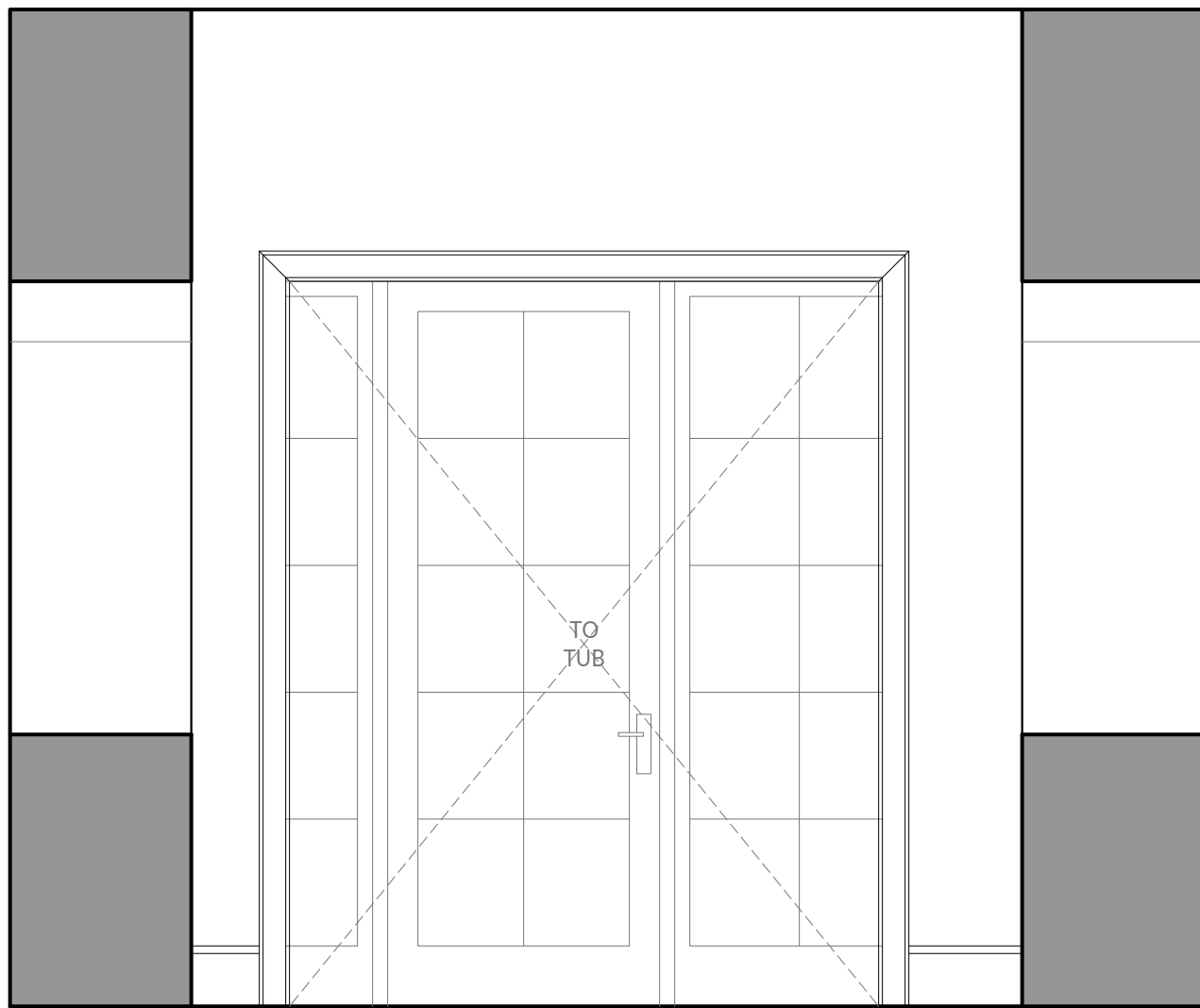
2 PRIMARY BATHROOM SCALE: 0' - 1/2" = 1' - 0"
